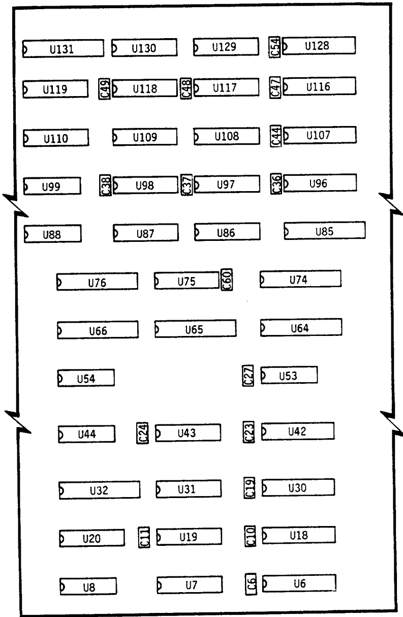
Figure 4. Circuit Card Assembly, Input/Output (A3) (Sheet 3 of 5)
