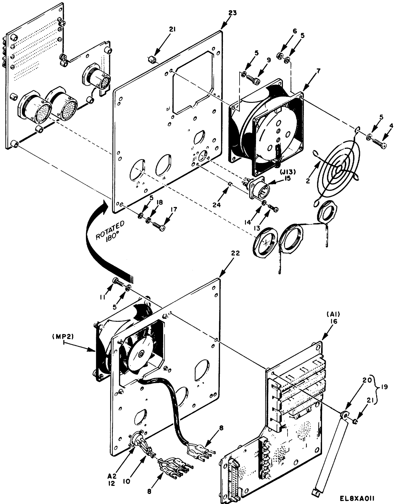
Figure 11. Rear Panel Assembly (A5)
