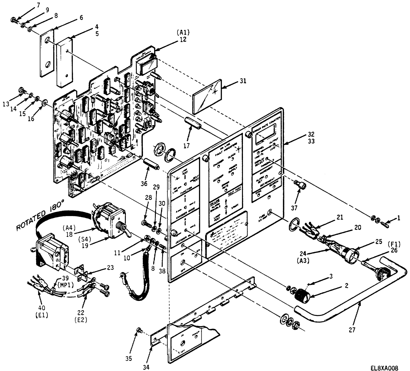
Figure 8. Front Panel Assembly (A6)
